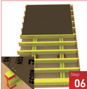
Fix plywood onto secondary beams by using screws or nails
