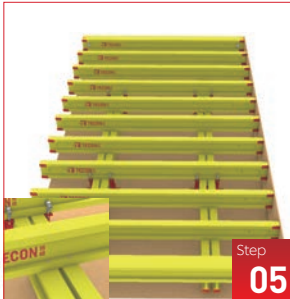
Fix other secondary beams onto main beams by using screws or nails at flange position until completion
